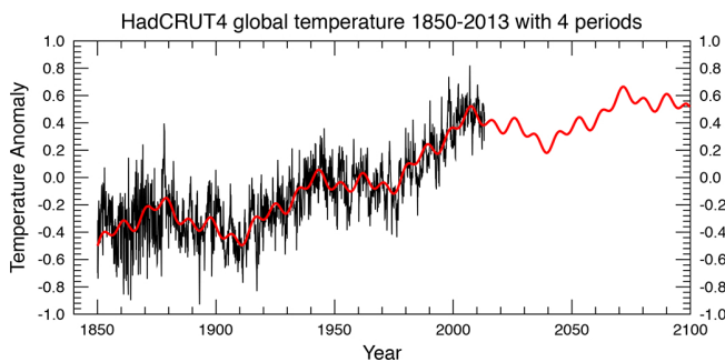
Figure 4. HadCRUT4 monthly averages of global temperature anomalies compared with a simple model consisting of a linear trend ( 0.0047\text{ }^{\circ}\text{C yr}^{-1} ) and four harmonic components with periods 155, 66, 21.6 and 9.14 yr.
